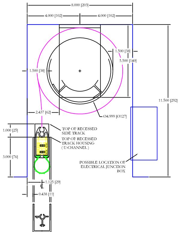
PLACEMENT OF 5" ROLLER, 5-1/2" ROLLER MOUNTING BRACKET AND RECESSED SIDE TRACK
